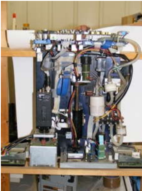
Complete Head Assembly including Bearings, Fiducial camera, Z-Axis boards etc.
